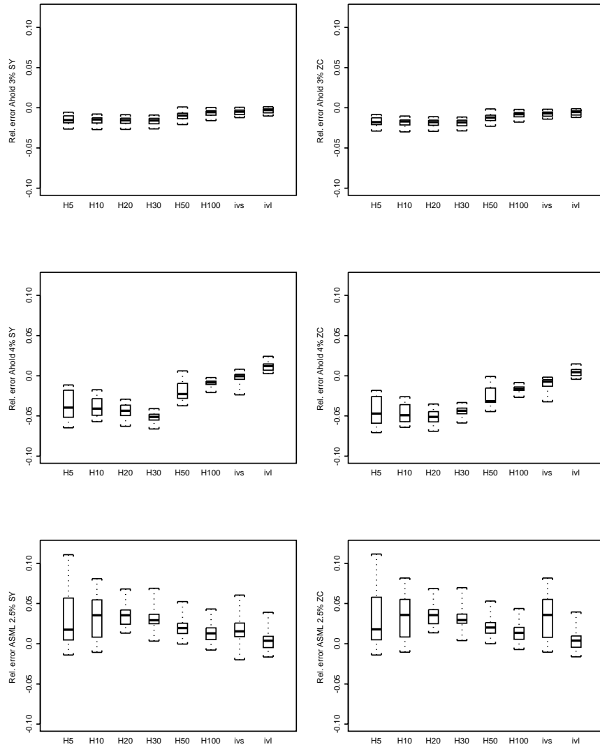
Figure 10: Boxplots of relative error of theoretical valuation.
